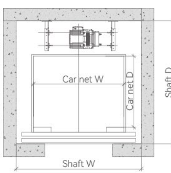
SHAFT LAYOUT
