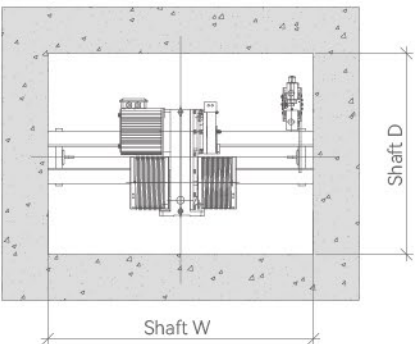
TOP FLOOR LAYOUT
