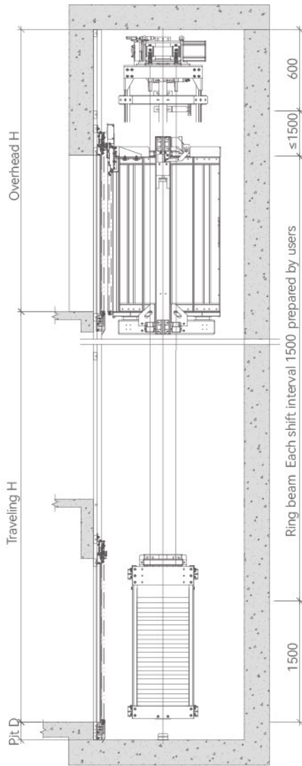
SHAFT VERTICAL SECTION
