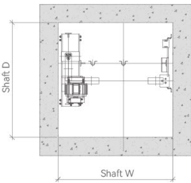
TOP FLOOR LAYOUT
