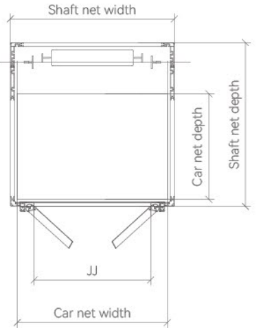
SHAFT LAYOUT
