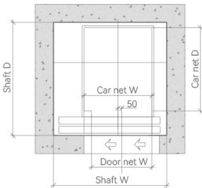
SHAFT LAYOUT
