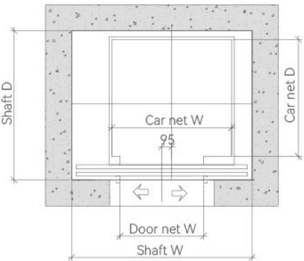
SHAFT LAYOUT
