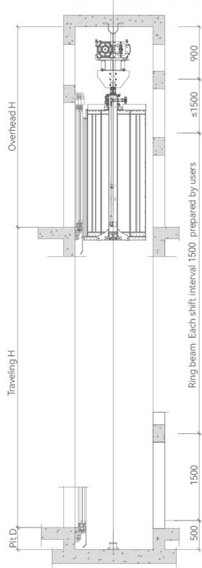
SHAFT VERTICAL SECTION
