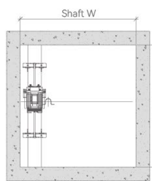
TOP FLOOR LAYOUT
