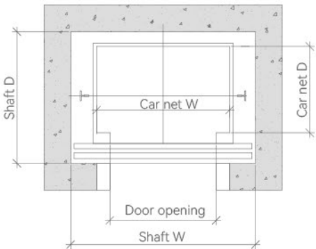
SHAFT LAYOUT
