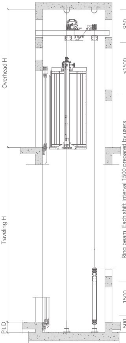
SHAFT VERTICAL SECTION
