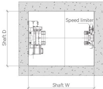
TOP FLOOR LAYOUT
