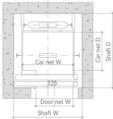
SHAFT LAYOUT
