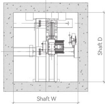
TOP FLOOR LAYOUT
